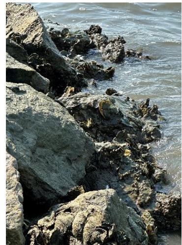
Fig 15. Low-water zone of a rock sill where oyster growth is high.
