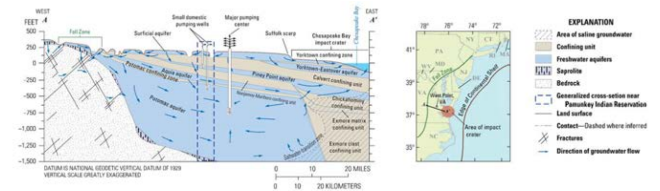
Figure 18. Generalized hydrogeologic cross section and directions of groundwater flow in the Virginia Coastal Plain under current conditions. Adapted from Foster et al, 2024.
