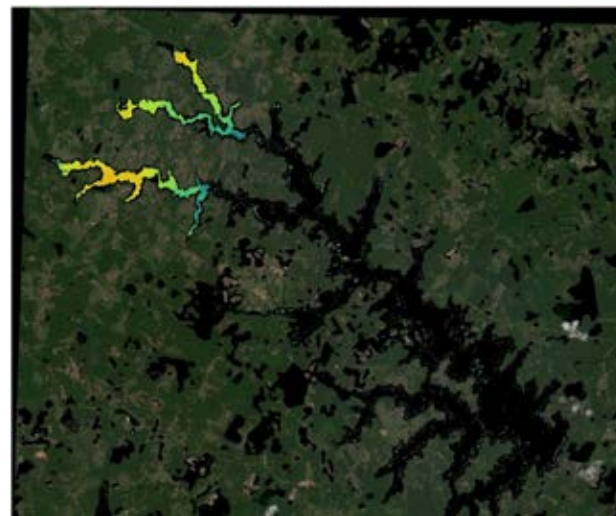
Figure 27b. Satellite image of a bloom in Lake Anna's upper north waters on 8/23/23. Data source: SENTINEL-2A MSI, Courtesy Copernicus Program, modified by NOAA CoastWatch.
