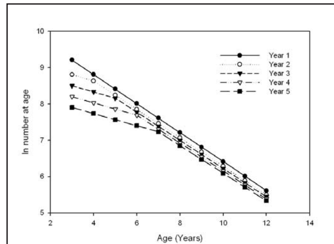
Figure 4. Non-equilibrium cross-sectional catch curves over a series of years showing a consistent 20% decrease in recruitment every year. Here total mortality ( Z ) is constant over all ages and all years and the departure from linearity is due to changing recruitment. The slope to the right of the bend reflects the true mortality rate. For clarity, each successive year's catch curve is displaced below the previous years curve. In practice, the height of the curve is determined in part by sampling effort.
