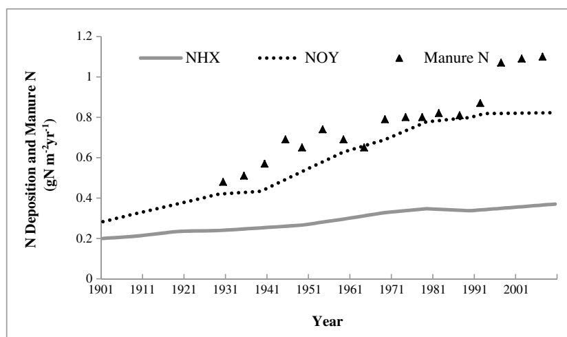
Figure 4. Nitrogen deposition ( \text{NH}_x ; reduced nitrogen and \text{NO}_y ; nitrogen oxides) and manure nitrogen production in eastern North America from 1901 to 2008.
