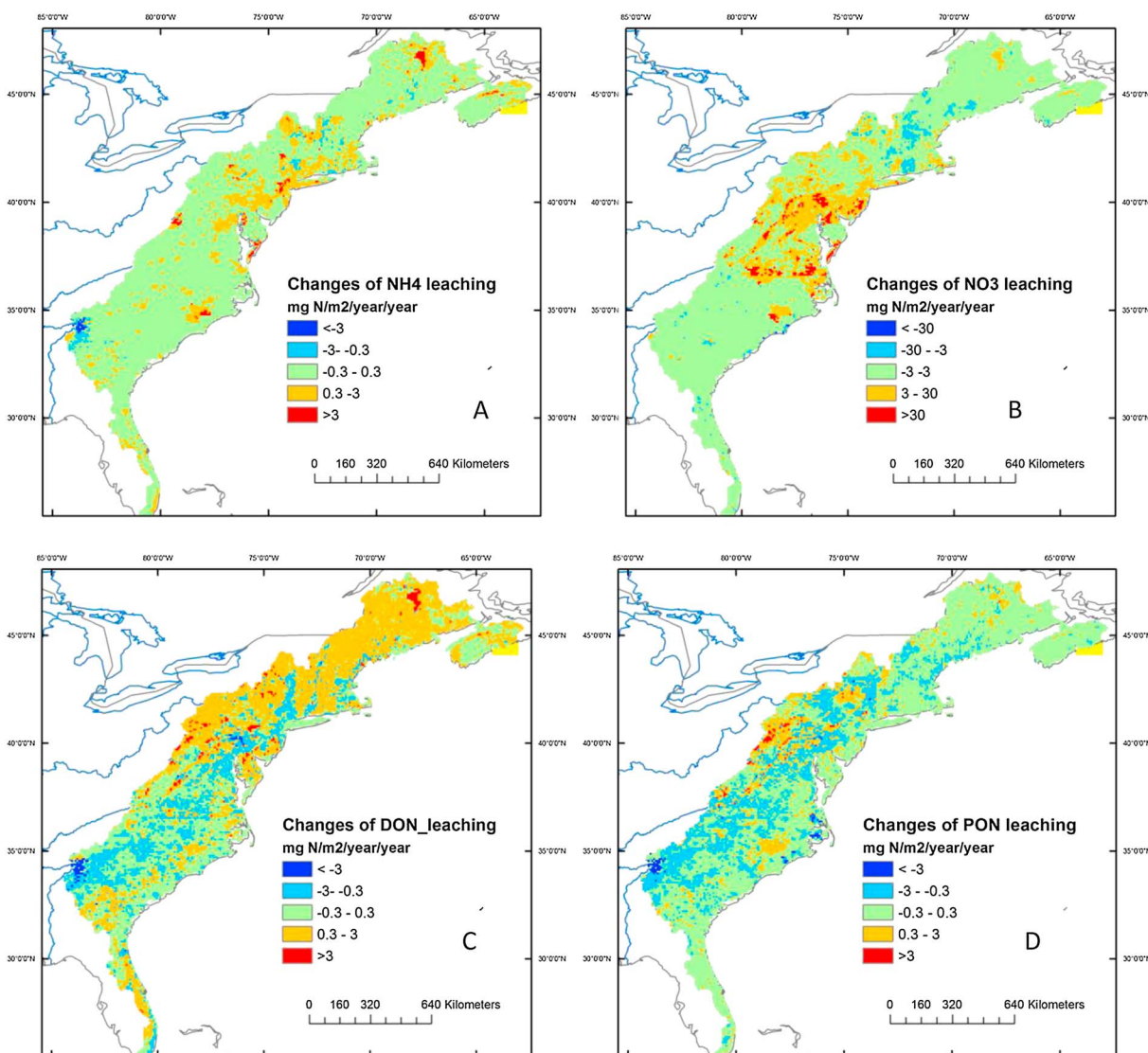
Figure 8. Spatial variability of the trend in annual mean nitrogen export across eastern North America during 1901–2008 ((a) \text{NH}_4 , (b) \text{NO}_3 , (c) \text{DON} , and (d) \text{PON} ).
