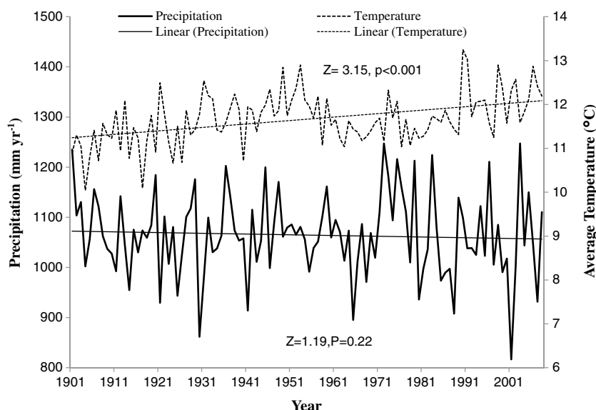
Figure 3. Precipitation and temperature changes in eastern North America from 1901 to 2008.
