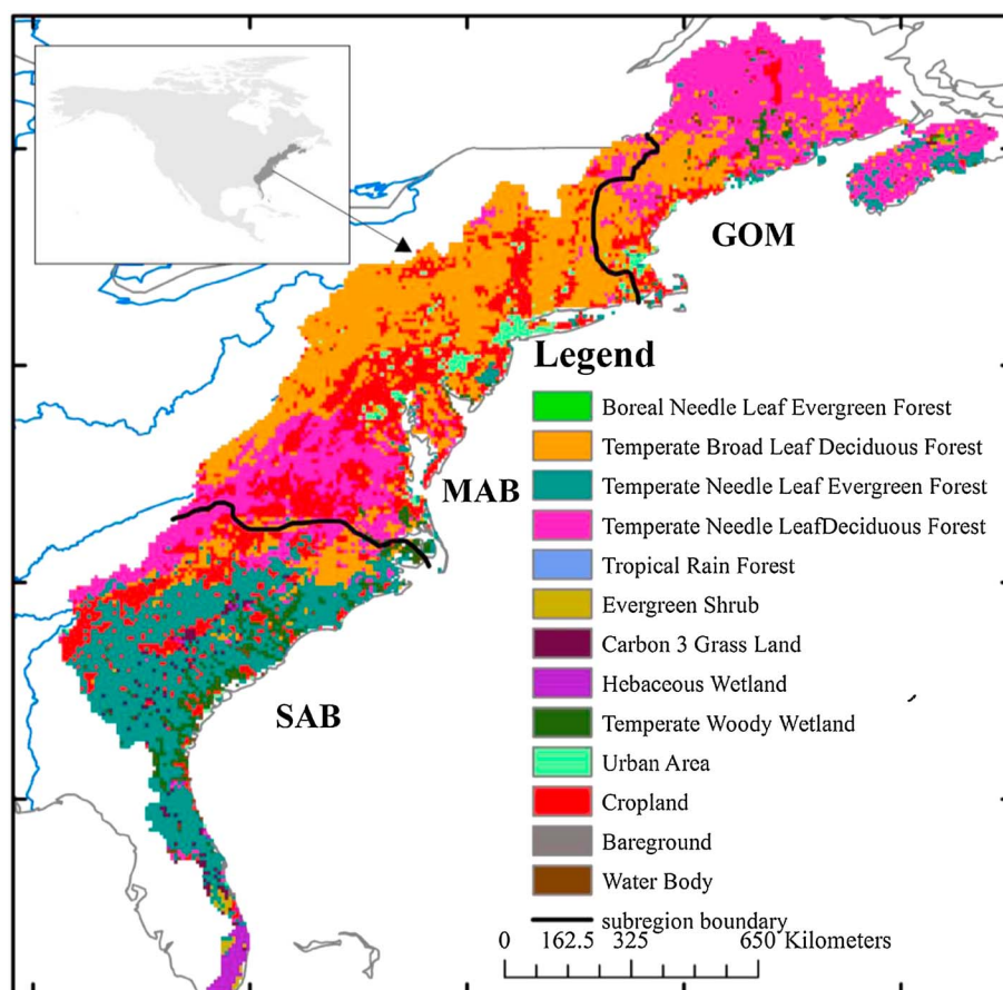
Figure 1. Location and land use types in eastern North America in 2005. Watersheds of the Gulf of Maine (GOM), Mid-Atlantic Bight (MAB), and South Atlantic Bight (SAB) are also delineated.
