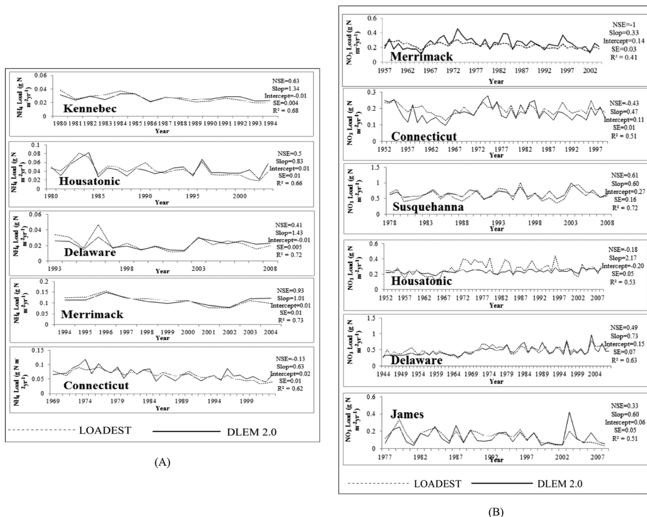
Figure 6. Comparison of nitrogen load estimated by Load Estimator (LOADEST) and DLEM 2.0 ((a) \text{NH}_4 , (b) \text{NO}_3 , (c) \text{DON} , and (d) \text{TON} ). NSE is the Nash-Sutcliffe model efficiency coefficient; slopes and intercept are for the linear regression between our simulations and LOADEST estimates; SE refers to standard error of the linear regression.
