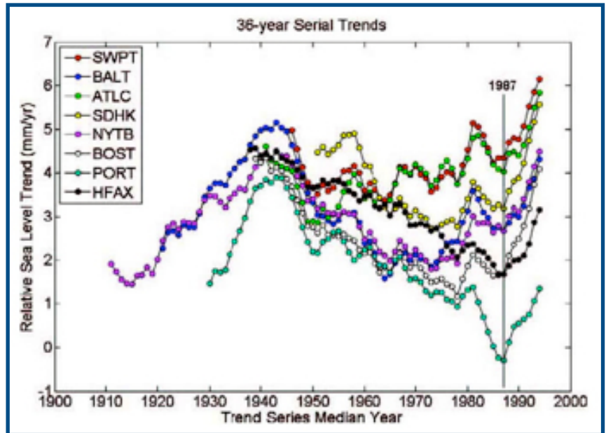
Abrupt Shift: The rate at which sea level is rising increased abruptly beginning in 1987 at all 8 stations along the northeastern U.S. coast: SWPT = Norfolk; BALT = Baltimore; ATLC = Atlantic City; SDHK = Sandy Hook, NJ; NYTB = New York; BOST = Boston; PORT = Portland, ME; HFAX = Halifax, Nova Scotia.
